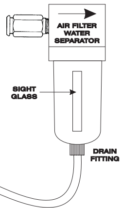
Figure 14 Air Filter Water Separator
