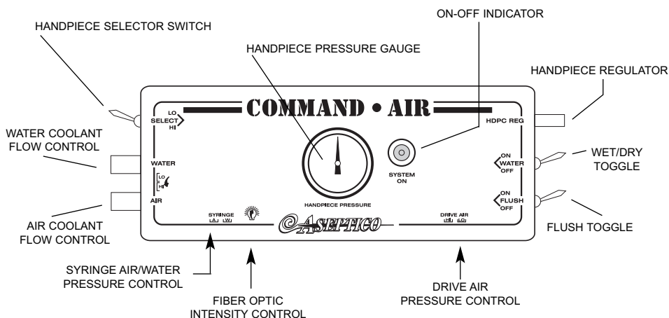
Figure 5 Handpiece Controls
