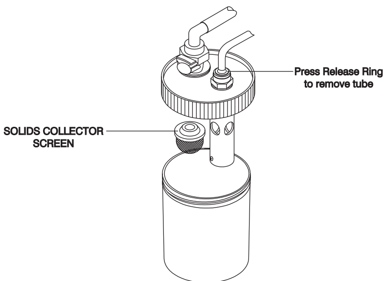
Figure 15 Solids Collector
